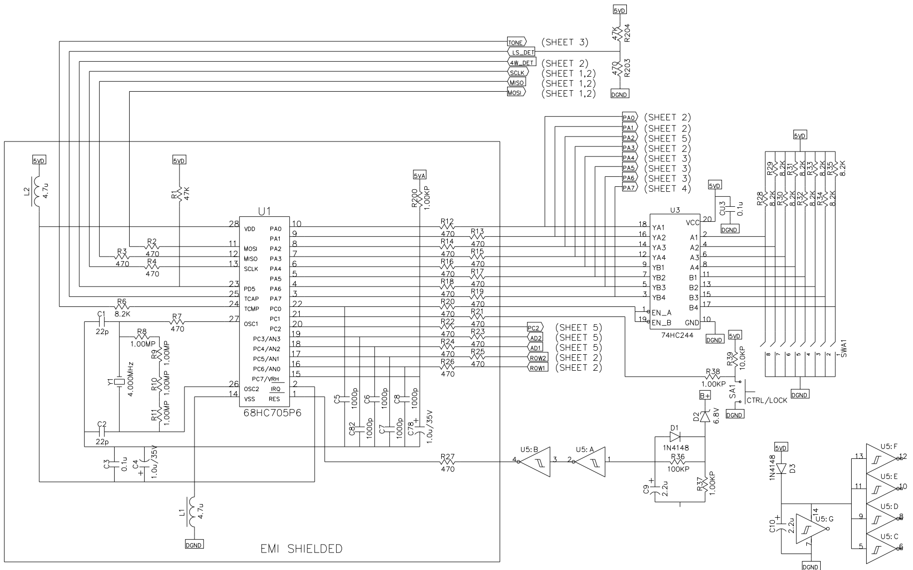
Tone Desk Set Microprocessor Section Schematic - Sheet 1
